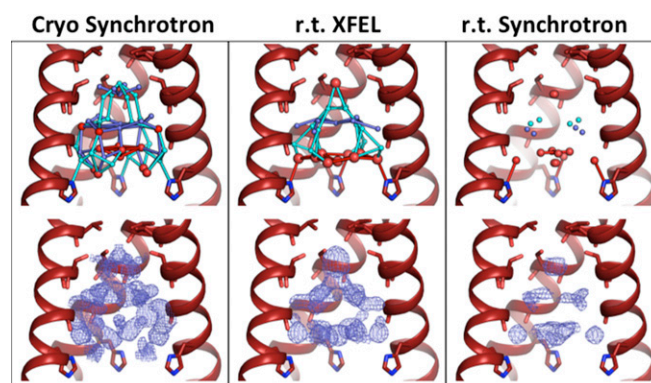
Fig. 1. Low-pH ( pH 5.5) structures of M2TM under cryogenic synchrotron (4QKC, Left), room temperature XFEL (5J0O, Center), and room temperature (r.t.) synchrotron (4QKM, Right) diffraction conditions. (Top) The front helix of each tetramer has been removed; waters are modeled as spheres, with red spheres representing full-occupancy waters and light and dark blue spheres as half-occupancy waters in alternate-occupancy networks A and B. Waters within hydrogen-bonding distance of each other are connected by sticks. The number of ordered waters decreases moving from Left to Right across the figure. (Bottom) Electron density for the pore solvent network (blue mesh) is shown to a contour of 0.5 \sigma . The largest amount of ordered density is present in the cryogenic synchrotron data collection condition. The volume and shape of the solvent density for the room temperature structures collected using XFEL and synchrotron sources are similar.
