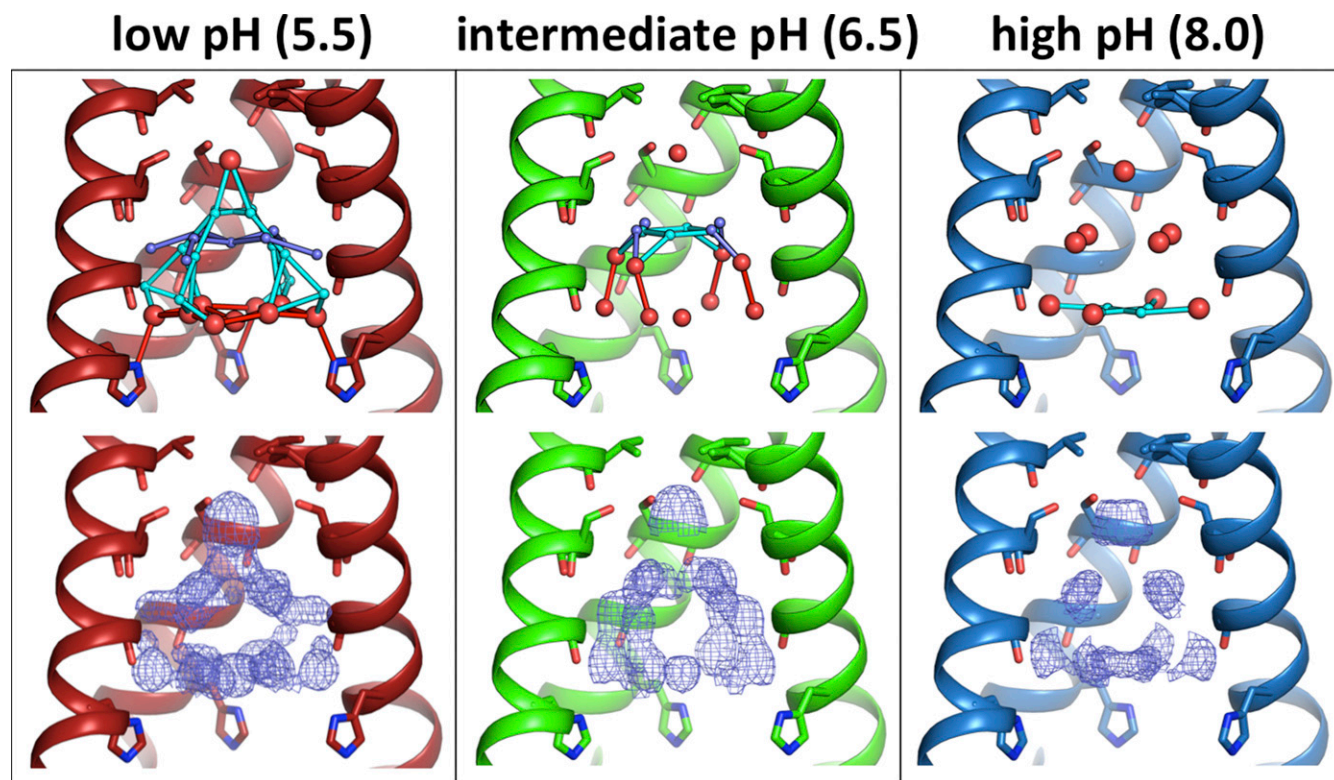
Fig. 4. Room temperature XFEL structures of M2TM under all pH conditions: low (pH 5.5, 5J00, red), intermediate (pH 6.5, 5U01, green), and high (pH 8.0, 5TTC, blue). Waters are shown as spheres (red, full occupancy; light and dark blue, half-occupancy); potential hydrogen bonds are shown as sticks. (Top) The most ordered waters are observed under the low-pH condition, with fewer waters present at intermediate pH and the smallest number of ordered waters at high pH. Moving from low to high pH, the number of half-occupancy waters decreases and the hydrogen-bonding network becomes less complex. (Bottom) Electron density for the pore solvent network (blue mesh) is shown to a contour of 0.5 \sigma . The same trend is observed from the electron density maps; the largest volume of solvent density is at low pH, and the smallest volume is at high pH.
